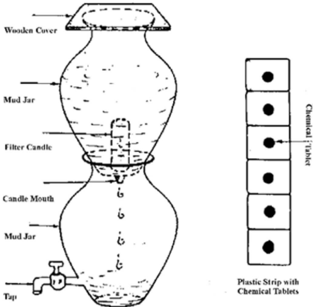
Figure 1(a) Arsenic removal Filter-Tablet system of School of Environmental Studies, Jadavpur University
